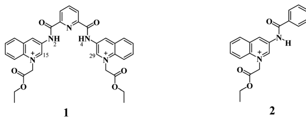
Scheme 1 Fluorescent receptors 1 and 2 employed in this study.
