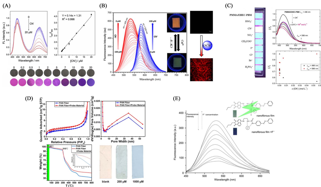
Fig. 20 Sensing properties of \text{CN}^- , F ^- -sensor (A) reprinted with permission from ref. 125. Copyright 2019, Elsevier. (B) Reprinted with permission from ref. 126. Copyright 2018, Elsevier. (C) Reprinted with permission from ref. 127. Copyright 2020, Elsevier. (D) Reprinted with permission from ref. 128. Copyright 2022, American Chemical Society. (E) Reprinted with permission from ref. 129. Copyright 2021, Huan Zhang et al.
