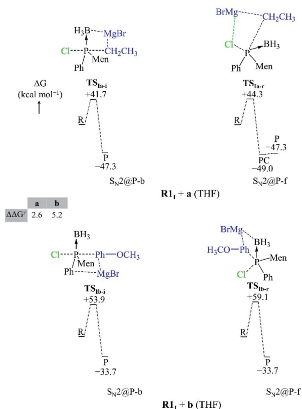
Fig. 3 Geometries of the TSs and PESs of the R1 1 + a and R1 1 + b S_N2@P reactions in the gas phase. The bond lengths/distances are in Å. The ΔG and ΔΔG ‡ are in kcal mol -1 .
