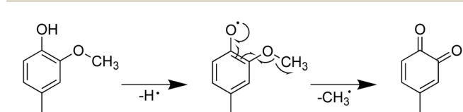
Scheme 1 Mechanism for the reaction between 2-methoxy-4-methylphenol and ROO • .
