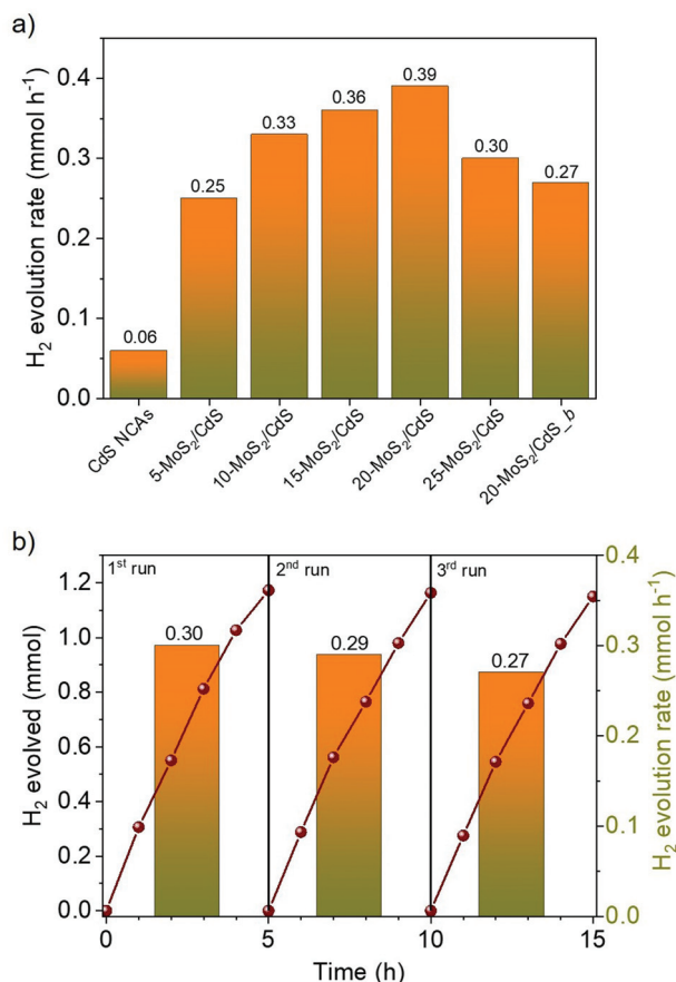
Fig. 4 (a) H 2 production rates for the mesoporous CdS and MoS 2 /CdS NCAs. The H 2 evolution rate of the catalyst with 20 wt% bulk MoS 2 (20-MoS 2 /CdS_b) is also given. (b) Photocatalytic recycling tests of the 20-MoS 2 /CdS NCAs. The columns show the H 2 production rates of the 5 h time intervals. Reaction conditions: 20 mg catalyst (or 30 mg for recycling study), 20 mL aqueous solution of 0.35 M Na 2 S and 0.25 M Na 2 SO 3 , 300 W Xenon light source with a cut-off filter ( \lambda \geq 420 nm), 20 \pm 2 °C.
