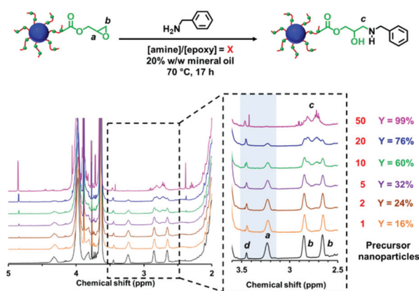
Fig. 2 1 H NMR spectra recorded in CD 2 Cl 2 for P(LMA 50 -stat-GlyMA 9 )-PMMA 67 before (black spectrum) and after reaction with benzylamine at 70 °C for 17 h at 20% w/w solids when using an [amine]/[epoxy] molar ratio (X) of 1 (orange spectrum), 2 (brown spectrum), 5 (purple spectrum), 10 (green spectrum), 20 (blue spectrum) and 50 (pink spectrum), respectively. Expansion of the 2.5–3.6 ppm region confirms the systematic loss of epoxy groups (note the gradual attenuation of methine signal a and the evolution of a new methylene signal c on increasing the [amine]/[epoxy] molar ratio. In each case, the epoxy loss (Y%) was determined by comparing the satellite signal d assigned to the PMMA backbone at 3.43–3.47 ppm to the methine signal a corresponding to the epoxide ring at 3.12–3.30 ppm.
