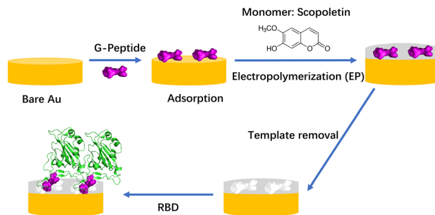
Scheme 1 Workflow of MIP preparation and binding of RBD (PDB code: 6MOJ). It was assumed that the template G-Peptide (GFNCYFP) was adsorbed “horizontally” via Cys488 on the bare gold.
