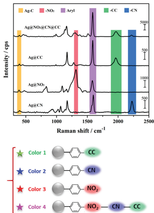
Fig. 5 SERS spectra of the three single layer-SERS tags and multilayer-coated Ag@NO 2 @CN@CC NPs. The excitation wavelength was 638 \text{ nm} , and the exposure time was 2 \text{ s} . The molecular structures of the three Raman reporters derived from aryl diazonium salts and the multilayer-coated Ag@NO 2 @CN@CC NPs are illustrated below.
