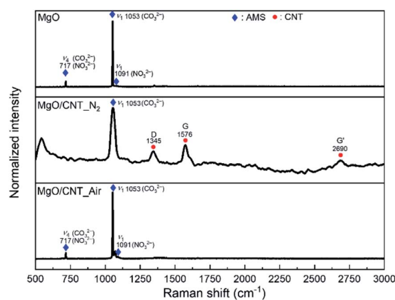
Fig. 5 Raman spectra of \text{MgO} -based sorbents after 30 cycles of carbonation–calcination reactions.
