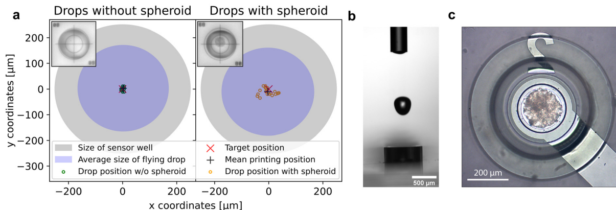
Fig. 2 Accuracy and precision of the impact position regarding single spheroid deposition. (a) Impact position of individually printed drops ( n_{w/o} spheroid = 30, n_{with} spheroid = 23) in relation to an initially determined reference printing position (red cross). The mean impact position is displayed by the black cross. The insets show exemplary drops of pure PBS or of PBS containing a spheroid positioned on the NBS 1952 resolution test target slide (crosshair of the slide has a length and width of 610 \mu\text{m} ). For clarity, the largest mean diameter of a free-flying droplet just above the sensor well is shown in blue and the size of the sensor well is shown in grey. (b) Side view of a PBS drop ejected from the nozzle and falling into the sensor well. (c) Exemplary image of a spheroid successfully deposited into a sensor well.
