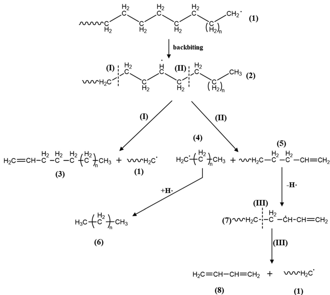
Scheme 1 Fundamental reactions for the thermal decomposition of PE leading to alkanes (6), alkenes (5) and alkenediene (8). Arabic numerals indicate chemical species that form during the pyrolysis of PE, while Roman numerals indicate the occurrence and position of the scission of chemical bond.
