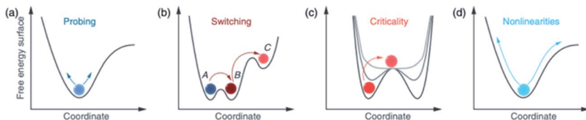
Fig. 1 Illustration of the range of applications of increasingly intense short light pulses to material systems. (a) Probing quasi particle interactions. (b) A more intense pulse populates the degenerate g.s. or moves the system to a metastable state. (c) Modifying the PES to induce nonequilibrium critical behavior. (d) Moving out of the harmonic region to create nonlinearities. (Figure reprinted with permission from A. De La Torre, D. M. Kennes, M. Claassen, S. Gerber, J. W. McIver and M. A. Sentef, Rev. Mod. Phys. , 2021, 93 , 041002. Copyright 2021 by the American Physical Society). 4
