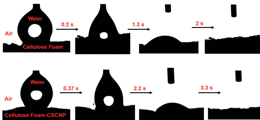
Fig. 5 Water contact angle measurements reveal the hydrophilic nature of the CF and CF-CSCNP surfaces, and indicate the water soaking behaviors with respect to time, captured through different image frames using a contact angle meter.
