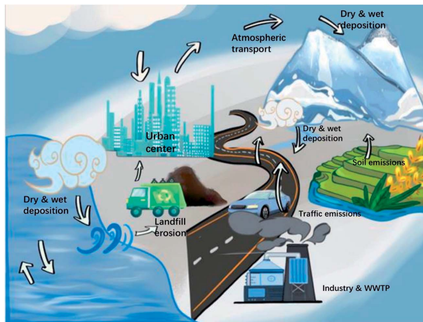
Fig. 4 Sources, transport and fates of MPs in the atmosphere.
