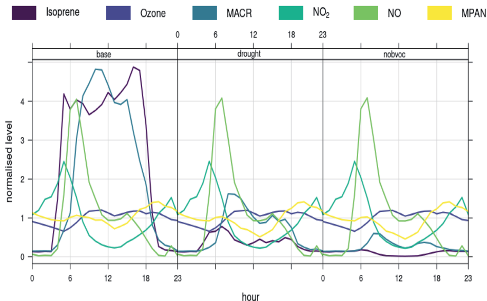
Fig. 8 Normalized mean diurnal variations for MACR, MPAN, isoprene, ozone, NO and \text{NO}_2 in July for different scenarios at HP. Time in hours on the x-axis refers to local time.
