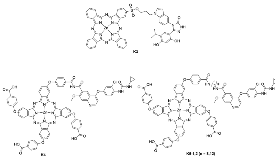
Fig. 13 Top: Pc–ganetespi conjugate; bottom: Pc–lenvatinib conjugates. K4 and the K5 series are statistical mixtures of isomers with all combinations of substitution in the \beta -positions of the isoindole units of the Pcs.
