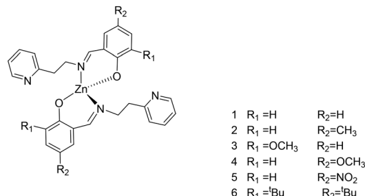
Scheme 2 Structures of the homoleptic Zn(II) complexes 1 – 6 .
