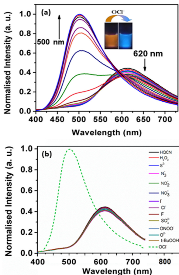
Fig. 4 (a) Fluorescence emission of HQCN (10 \mu\text{M} in \text{CH}_3\text{OH}-\text{H}_2\text{O} ; 1/4, v/v in the presence of HEPES buffer (10 mM) solution at \text{pH} = 7.2 ) upon the gradual addition of \text{OCl}^- (0 to 5 equivalents). Ratiometric spectra of HQCN were observed after the addition of \text{OCl}^- , where the \lambda excitation was 370 nm. The fluorescence emission peak at 620 nm gradually decreased and the peak at 500 nm gradually increased after the addition of \text{OCl}^- . Inset shows the visible emission of HQCN in the absence and presence of 2 equivalents of \text{HOCl} upon irradiation under UV light. (b) Fluorescence emission spectra of HQCN (10 \mu\text{M} in \text{CH}_3\text{OH}-\text{H}_2\text{O} ; 1/4, v/v in the presence of HEPES buffer (10 mM) solution at \text{pH} = 7.2 ) upon addition of different guest analytes (0 to 5 equivalents). Apart from \text{OCl}^- , no significant change was observed for other guest analytes.
