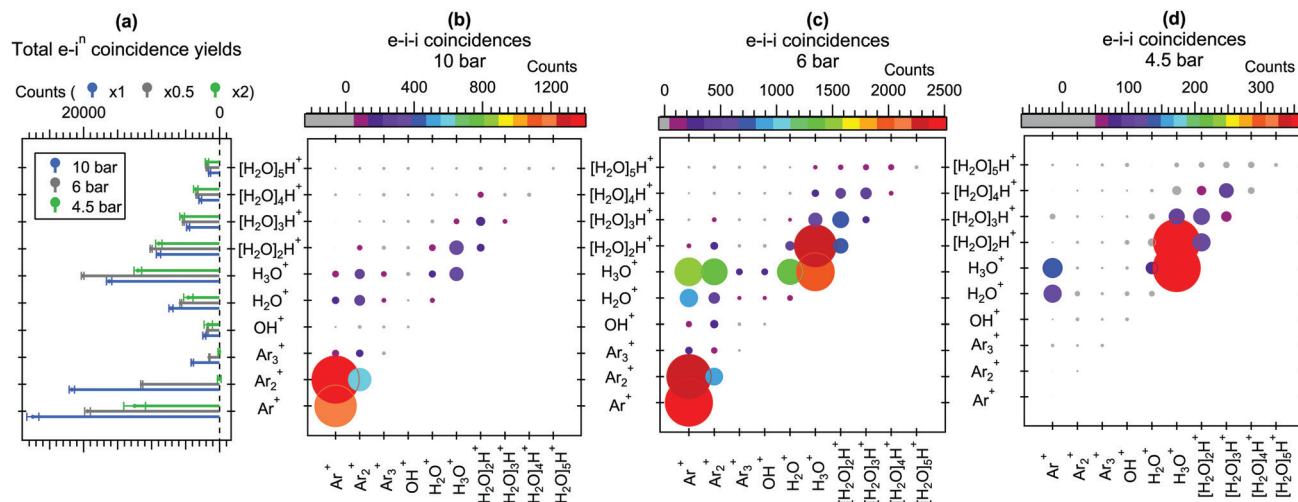
Fig. 3 (a) Total e-i 2 coincidence yields. The intensities at different pressures are scaled to comparable [\text{H}_2\text{O}]_n\text{H}^+ intensities for better comparison. (b-d) e-i-i coincidences at 10 bar, 6 bar and 4.5 bar expansions.
