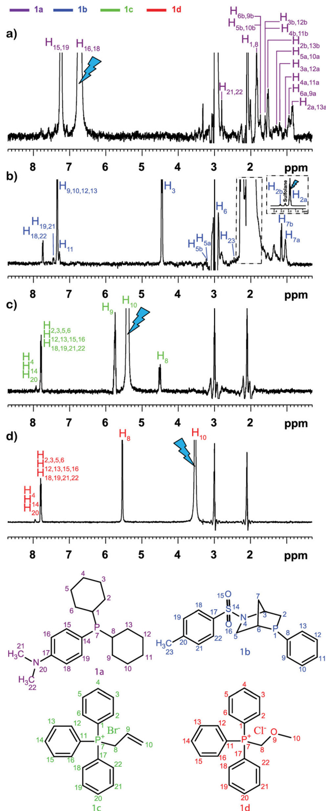
Fig. 4 Multiplier selective excitation 1D 1 H NOESY spectra of a phosphorus-based compound mixture (20 mM) dissolved in sulfolane/DMSO- d 6 (7 : 3 v/v) (a–d), t m = 1 s, at 258 K, at 500 MHz ( 1 H). The initial selective inversion pulses excite: (a) H 16,18 (1a), (b) H 2a (1b), (c) H 10 (1c), and (d) H 10 (1d) proton resonances. Reproduced with permission from ref. 69, © 2020 American Chemical Society.
