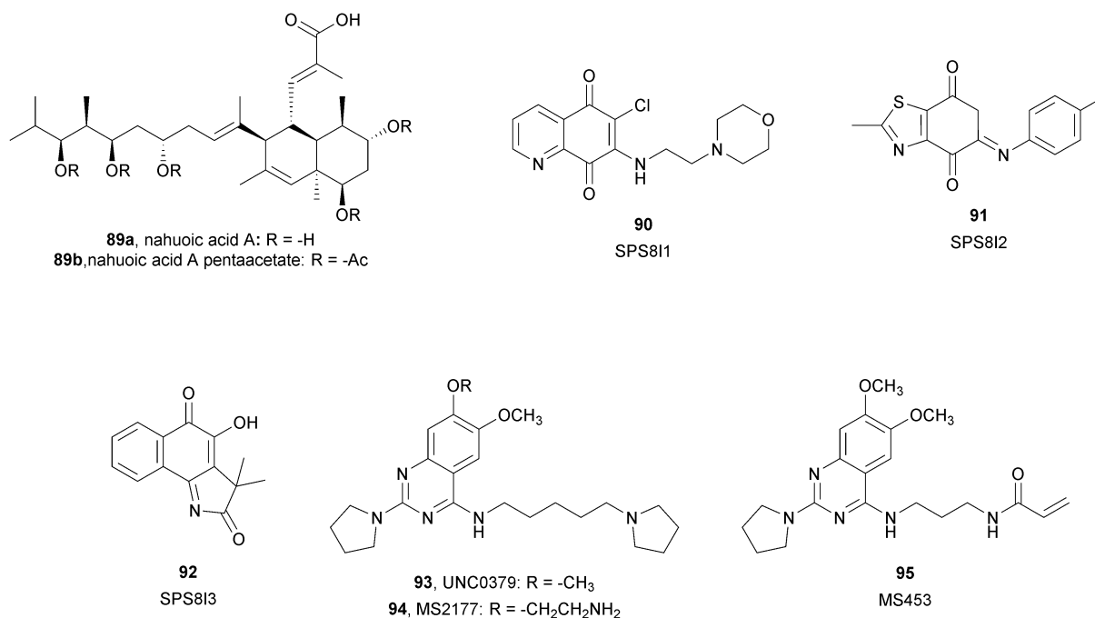
Fig. 24 SETD8 inhibitors.
