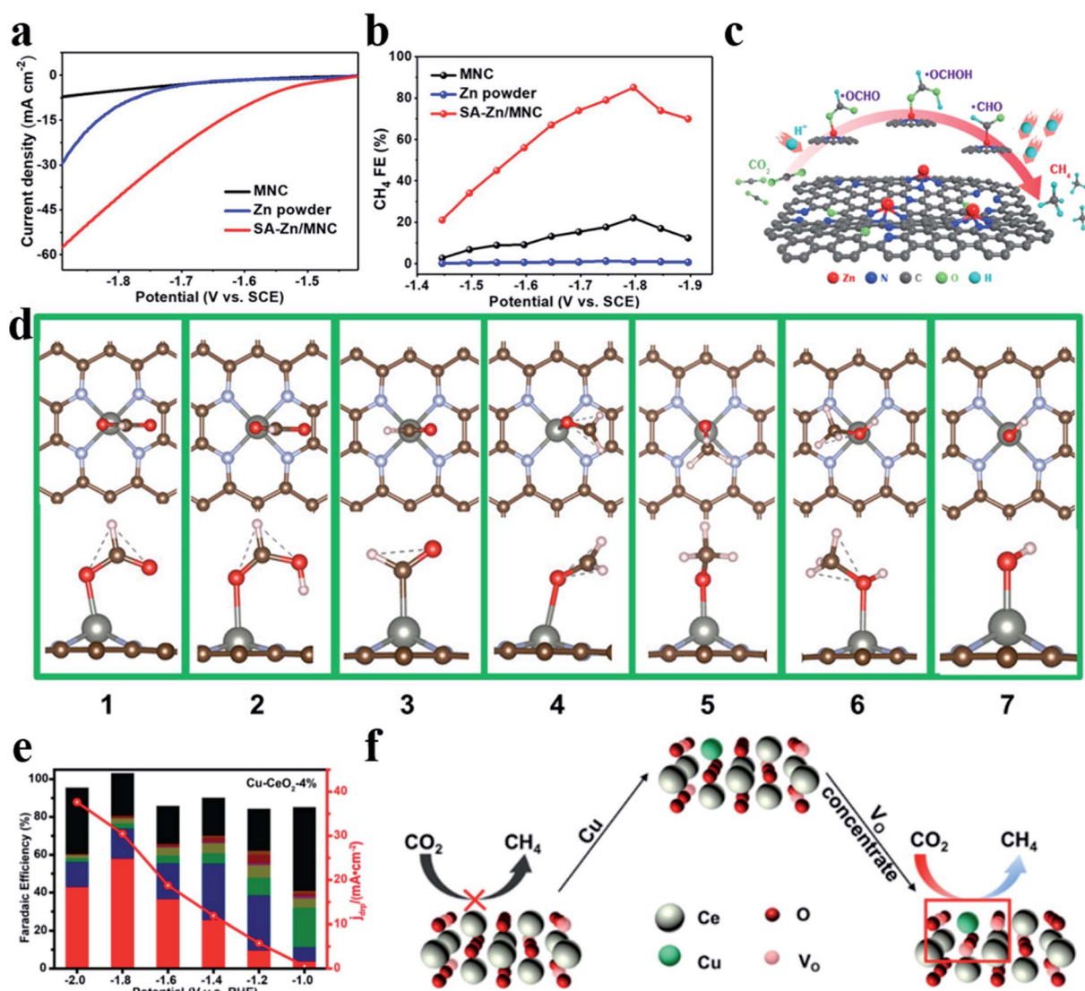
Fig. 10 (a) Polarization curves for MNC, Zn powder, and SA-Zn/MNC. (b) FEs for the electrochemical CO 2 RR to CH 4 at different applied potentials. (c) CO 2 RR pathway for single Zn atoms to produce CH 4 . (d) The most stable structure. The red and pink balls represent O and H atoms, respectively. Reproduced with permission from ref. 106. Copyright (2020) American Chemical Society. (e) Faradaic efficiencies (bars, left y-axis) and the deep reduction product current density ( j_{drp} , red curve, right y-axis) of Cu-CeO 2 -4%. The red column represents CH 4 . (f) Effect of oxygen vacancies on the CO 2 RR. Reproduced with permission from ref. 107. Copyright (2018) American Chemical Society.
