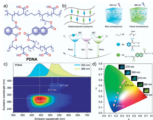
Fig. 9 (a) Chemical structure of PDNA . (b) Schematic illustration of the proposed mechanism of colour-tunable URTP of PDNA . (c) Excitation-phosphorescence mapping of PDNA under ambient conditions; the inset displays the phosphorescence spectra excited at 254 nm (blue) and 365 nm (yellow). (d) CIE chromaticity diagram for PDNA with excitation varied from 270 to 370 nm; the inset shows the UOP photographs of PDNA excited at various wavelengths. Reproduced with permission from ref. 110. Copyright 2020, Springer Nature Limited.
