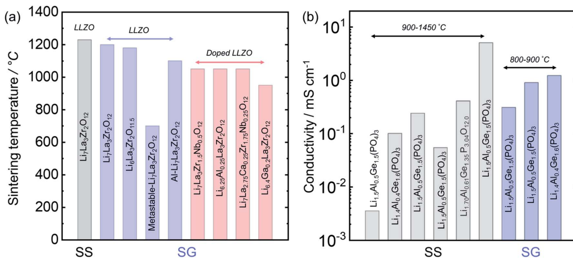
Fig. 11 Influence of synthesis route on the sintering temperature and conductivity of cubic Li 7 La 3 Zr 3 O 12 and Li 1+x Al x Ge 2-x (PO 4 ) 3 . (a) The sintering temperature for sol-gel (SG) route 41,140,219,226 is lower than solid-state (SS) synthesis, 37 which further decreases with substitution. 224–227 (b) Ionic conductivities of Li 1+x Al x Ge 2-x (PO 4 ) 3 synthesized via SS 139,231–234 and SG methods. 45,49,235
