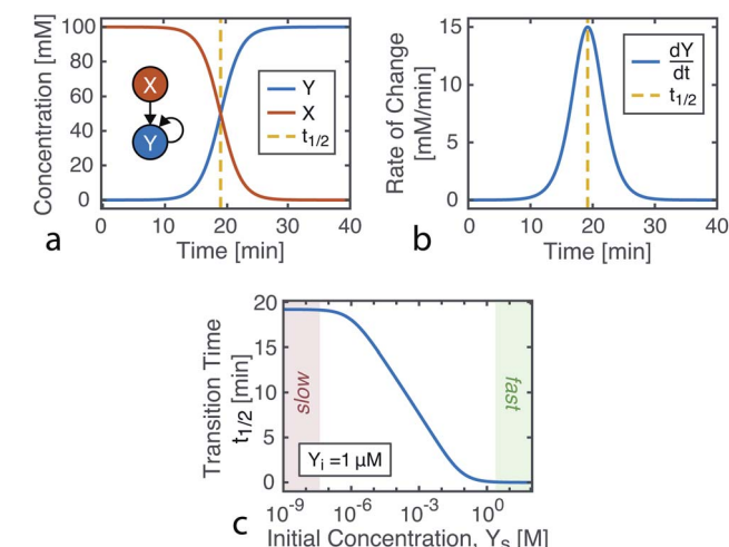
Fig. 1 Kinetics of autocatalysis. (a) Reagent and autocatalytic product evolution over time for X_0 = 100 mM, Y_0 = 1 \mu M, and k = 0.1 (eqn (4)). (b) Rate of product concentration change over time for the reaction simulated in a, showing the accelerated production typical of an autocatalytic process. (c) The time to transition as the input catalyst concentration ( Y_0 ) is varied about a constant: Y_0 = Y_i + Y_s with Y_i = 1 \mu M, X_0 = 100 mM, and k = 0.1 .
