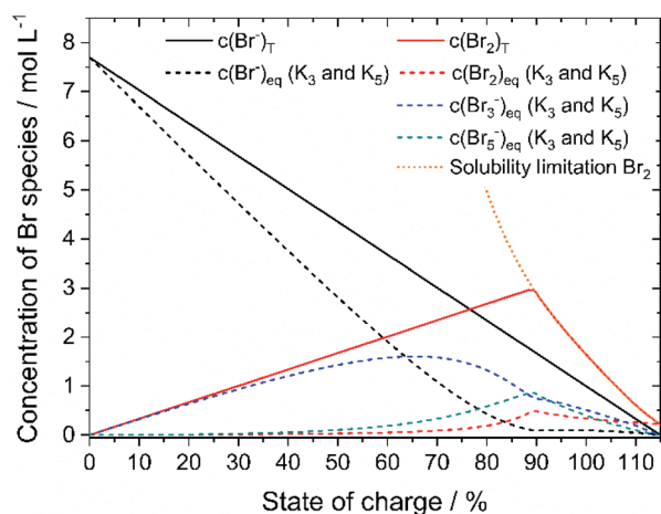
Fig. 7 Plot of the theoretical concentration of \text{HBr}_{\text{T}} , \text{Br}_{2,\text{T}} , \text{Br}_{3,\text{eq}}^- , \text{Br}_{5,\text{eq}}^- with K_3 = 16 \text{ L mol}^{-1} and K_5 = 37 \text{ L}^2 \text{ mol}^{-2} including bromine solubility limit.
