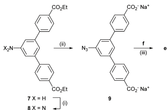
Scheme 4 Synthesis of the stopper 9 in 2 steps and CuAAC “click” reaction providing e . Reagents and conditions: (i) \text{TMSN}_3 , \text{tBuONO} , DMF, 0 °C to rt, 6 h, 98%; (ii) NaOH, THF–MeOH–H 2 O (4 : 4 : 1), 50 °C, 1 h, 86%; (iii) \text{CuSO}_4 \cdot 5\text{H}_2\text{O} , sodium ascorbate, H 2 O–MeOH (2 : 1), rt, 1 h, 65%.
