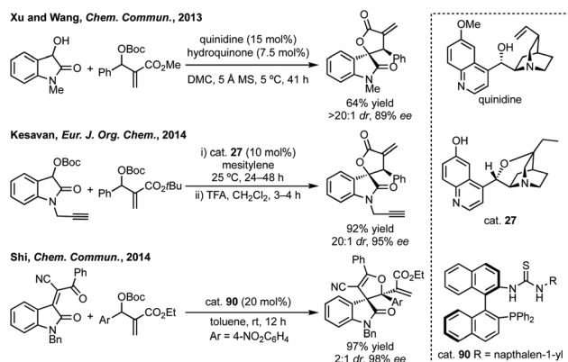
Scheme 60 Selected advances in the use of MBH carbonates to form spirocyclic lactones and spiroTHF oxindoles.
