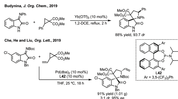
Scheme 42 Selected examples of 3,2'-spirocyclic oxindole synthesis by cyclopropane ring expansion.
