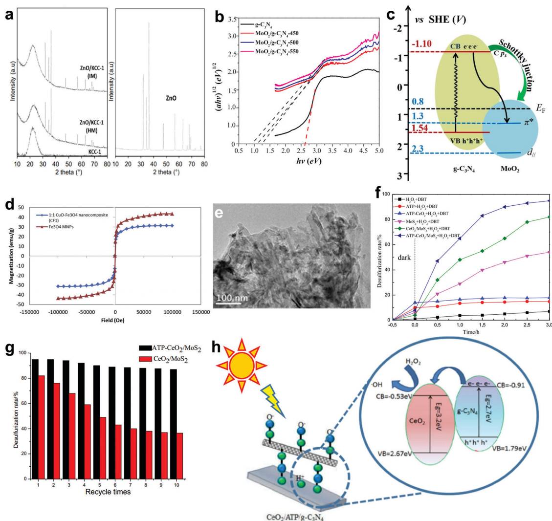
Fig. 21 (a) XRD spectra of ZnO/KCC-1(IM), ZnO/KCC-1(HM), KCC-1 and ZnO. Reprinted with permission. 231 Copyright 2020, Springer Nature. (b) Graph of (ah\nu)^{1/2} versus photon energy for g-C 3 N 4 and MoO 2 /g-C 3 N 4 with different synthesis temperatures. (c) Electronic structure of MoO 2 /g-C 3 N 4 with the electron movement. Reprinted with permission. 232 Copyright 2018, Elsevier B.V. (d) Magnetic hysteresis loops of CuO-Fe 3 O 4 and Fe 3 O 4 . Reprinted with permission. 233 Copyright 2018, Elsevier Ltd. (e) TEM image of ATP-CeO 2 /MoS 2 . (f) DBT oxidation of various catalysts and (g) the recyclability test for ATP-CeO 2 /MoS 2 and CeO 2 /MoS 2 using H 2 O 2 . Reprinted with permission. 235 Copyright 2016, Elsevier B.V. (h) Reaction pathway of photocatalytic ODS using ATP-CeO 2 /g-C 3 N 4 and H 2 O 2 under visible light irradiation. Reproduced with permission. 237 Copyright 2017, Elsevier B.V.
