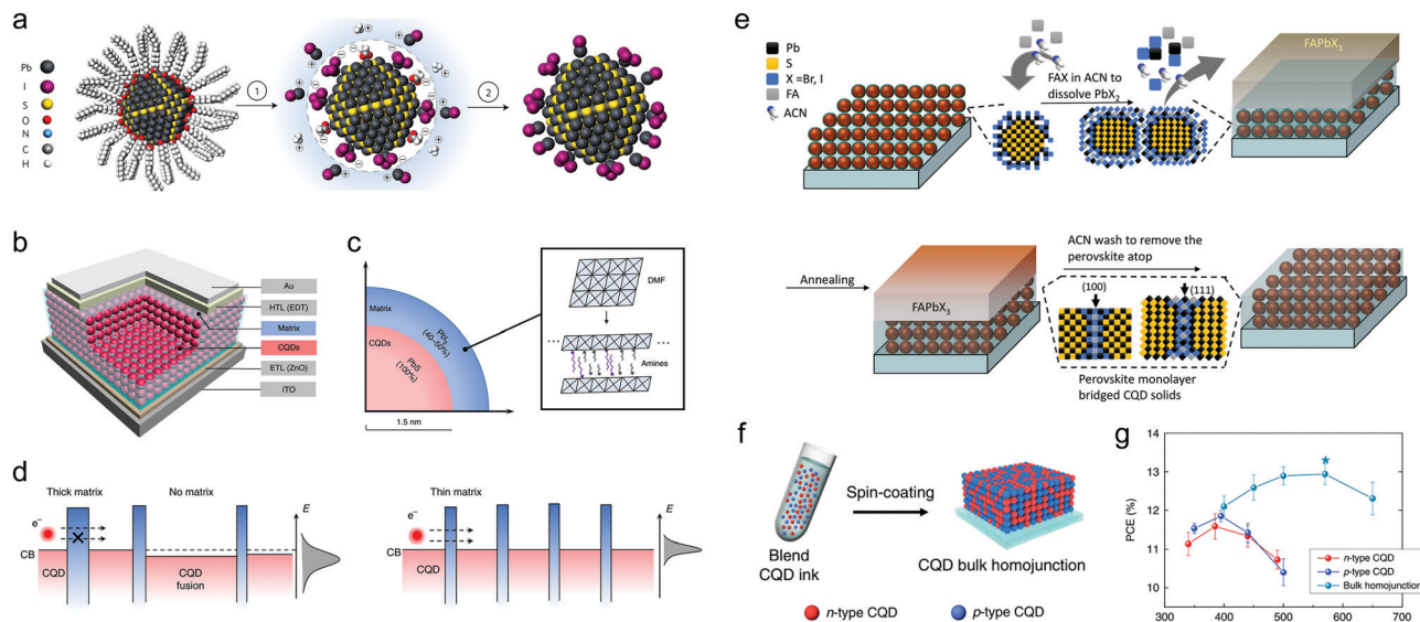
Fig. 3 (a) Solution-phase ligand exchange with metal halide precursors and ammonium acetate. Process 1 (ligand exchange): the bulky oleic acid ligands are replaced by the [PbX 3 ] - anions with the aid of ammonium protons. The CQD surface is stabilized by both [PbX] + and [NH 4 ] + . Process 2 (CQD precipitation): after ligand exchange, CQDs are precipitated via the addition of toluene, an anti-solvent, and are separated by centrifugation. Reprinted with permission from ref. 17. Copyright 2017, Nature Publishing Group. (b) Schematic diagram of the effective medium model of the CQD absorber in a solar cell, where CQDs (red) assemble in a matrix medium (blue). (c) The matrix consists of PbI 2 , which is enough to account for the formation of full monolayer coverage on the surfaces of PbS CQDs (bandgap ~1.3 eV and diameter ~3 nm). The dimensional structure of the matrix can be tuned using solvents. (d) The schematic diagram for the effect of homogeneity of the matrix on the structural and energetic order of CQD film. Confining the matrix dimensionality between the CQDs and improving its homogeneity throughout the film can increase the photocarrier diffusion length and reduces the V oc deficit. Reprinted with permission from ref. 43. Copyright 2018, Nature Publishing Group. (e) Schematic of the formation of monolayer perovskite bridges among the QDs. The perovskite matrix is formed first by soaking the pre-exchanged CQD films in a FAX (X = Br, I) solution, where the FAX solution dissolves the PbX 3 - ligands and perovskite grows between adjacent PbS CQDs. The films are annealed and then washed with acetonitrile to remove excess perovskite. Reprinted with permission from ref. 18. Copyright 2014, Elsevier. (f) The bulk-homojunction films were fabricated by depositing the blended CQD inks comprising n-type and p-type CQDs. (g) Thickness-dependent PCE for bulk-homojunction devices and n-type CQD devices. Bulk-homojunction devices enable the use of much thicker CQD films compared with the case of n-type CQD devices, indicating the increase of carrier diffusion length. Reprinted with permission from ref. 49. Copyright 2020, Nature Publishing Group.
