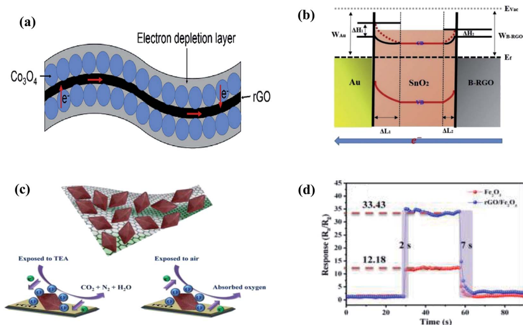
Fig. 19 (a) Schematic of the sensing mechanism of D-Co 3 O 4 /rGO composite 228 (reprinted from ref. 228, Copyright (2019), with permission from Elsevier). (b) Energy band diagram of the B-rGO/SnO 2 @Au heterostructure sensor 235 (reprinted from ref. 235, Copyright (2020), with permission from Elsevier). (c) Schematic diagram of the possible gas sensing mechanisms of rGO/ \alpha -Fe 2 O 3 nanocomposite. (d) Dynamic response–recovery curve (100 ppm TEA) of pure \alpha -Fe 2 O 3 spindles and rGO/ \alpha -Fe 2 O 3 nanocomposite at 280 °C (ref. 236) (reprinted from ref. 236, Copyright (2017), with permission from Elsevier).
