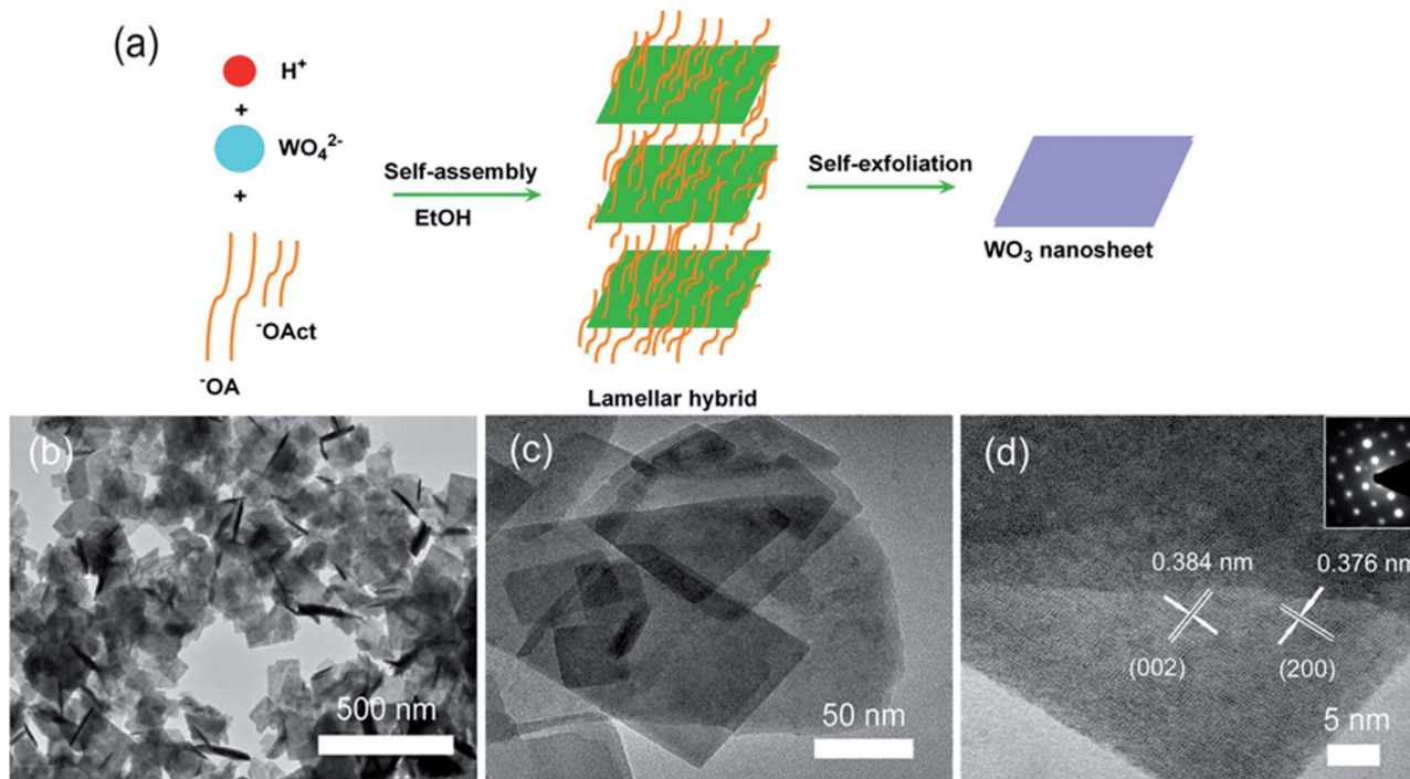
Fig. 3 (a) Schematic of self-assembly. (b–d) SEM, TEM, and HRTEM images of WO_3 nanosheets produced with a NaOct/NaOA mass ratio of 0.04. Reprinted with permission from ref. 53, copyright 2018, Elsevier.
