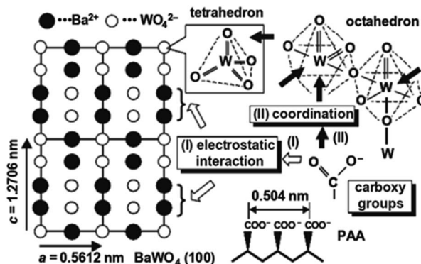
Fig. 4 Illustration of BaWO_4 (100) and the interaction with PAA molecules that leads to formation of octahedral WO_6 . Reprinted with permission from ref. 56, copyright 2006, John Wiley and Sons.
