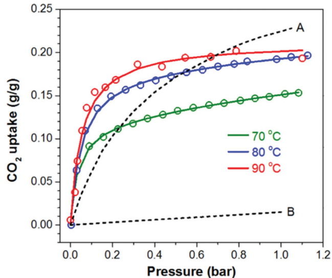
Fig. 15 CO 2 uptake isotherms of PEI–C 60 at 70 °C, 80 °C and 90 °C and compared to the absorption of CO 2 on (A) Mg-MOF-74 and (B) MOF-177, both at 90 °C. Reproduced from ref. 106 according to Creative Commons Attribution 4.0 International (CC BY 4.0).
