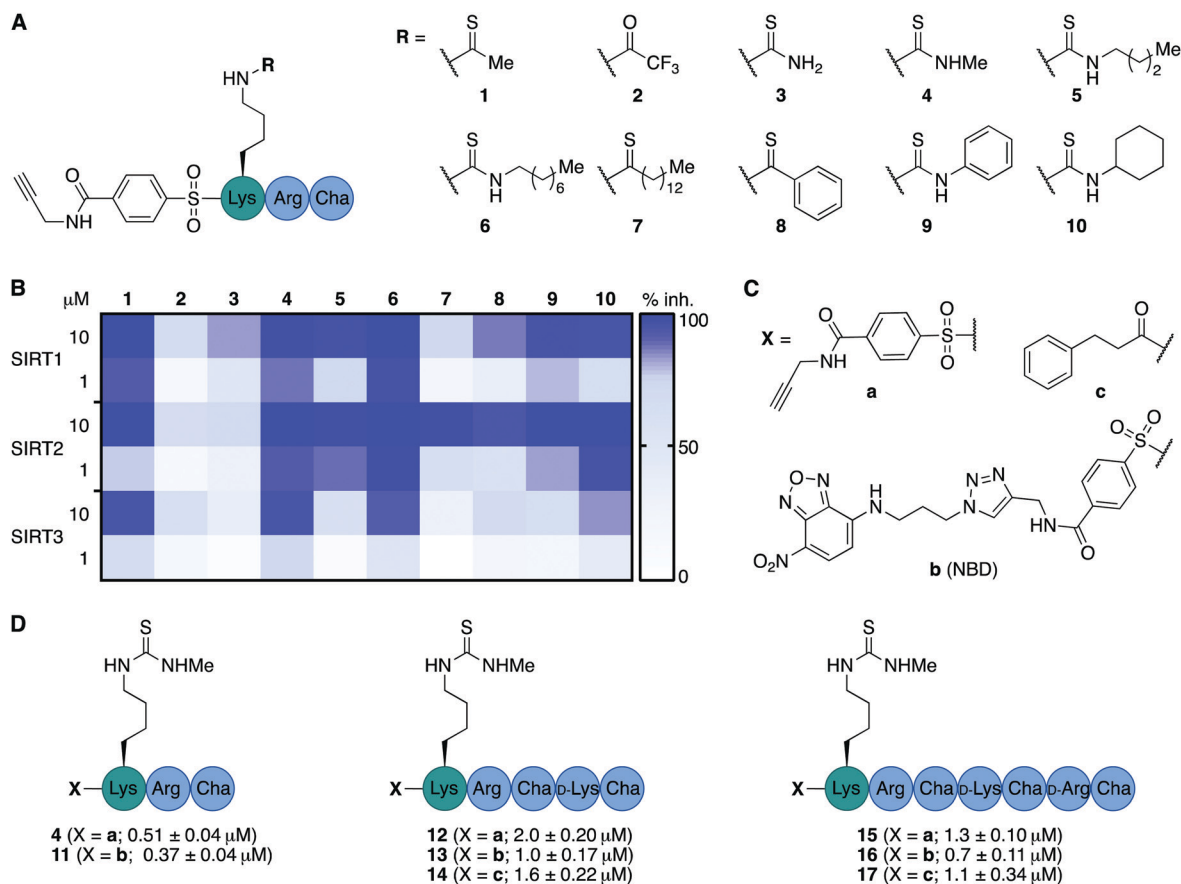
Fig. 2 Structure–activity relationship of inhibitors against SIRT1–3. (A) Structures of compounds 1–10. (B) Heatmap summarizing potencies of compounds 1–10 against SIRT1–3 based on % inhibition. All assays were performed at least twice in duplicate and the values can be found in Table S1 (ESI†). (C) Structures of N-terminal functional groups introduced in compounds 11–17. (D) Structures and \text{IC}_{50} values and standard deviations recorded for compounds 11–17 based on a minimum of two individual assays performed in duplicate. Further information and selectivity data can be found in Fig. S5 and Table S1 (ESI†).
