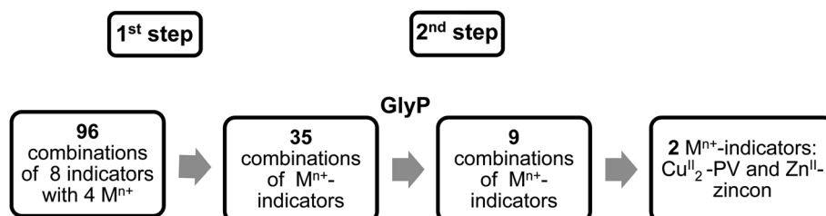
Fig. 3 Two-step screening procedure for the identification of \text{Cu}_2^+ -PV and \text{Zn}^{\text{II}} -zincon as metal-based GlyP probes.
