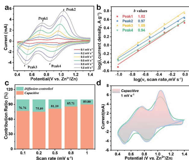
Fig. 3 (a) CV curves of the V 2 O 5 -YS cathode at various scan rates, (b) plots of log(current density) versus log(scan rate) based on the four main peaks, (c) ratio of capacitive and diffusion-controlled capacities at multiple scan rates, and (d) CV curve displaying the capacitive contribution (shadow area) to the total current at 1.0 mV s -1 .
