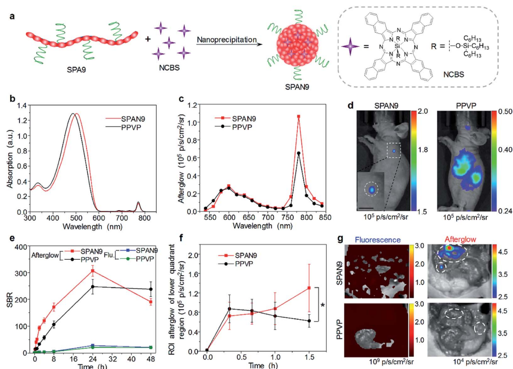
Fig. 3 (a) Schematic illustration for the preparation of SPAN9. (b) Absorption spectra of SPAN9 and PPVP in 1× PBS buffer (pH 7.4). (c) Afterglow spectra of SPAN9 and PPVP under the same mass concentration (130 μg mL -1 ). (d) Afterglow images of living mice after i.v. injection of SPAN9 or PPVP for 40 min. (e) SBRs for fluorescence and afterglow imaging of tumor in living mice injected with SPAN9 or PPVP as a function of post-injection time. (f) Afterglow intensities of the lower quadrant region of living mice after i.v. injection of SPAN9 or PPVP as a function of post-injection time. (g) Fluorescence and afterglow images of abdominal cavity of mice after skin resection at 1.5 h post-injection of SPAN9 or PPVP. White circles mark the position of tumors. *Statistically significant difference ( p < 0.05 , n = 3 ). Error bars represent standard deviations of three different measurements ( n = 3 ). Adapted from ref. 93. Copyright© 2018 Wiley-VCH Verlag GmbH & Co. KGaA, Weinheim.
