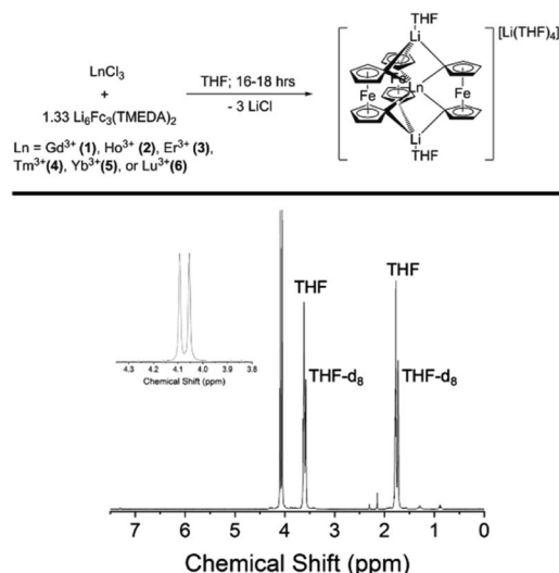
Fig. 1 (Top) Preparation of late \text{Ln} -[1]ferrocenophane compounds. (Bottom) ^1\text{H} NMR (400 MHz, \text{THF-d}_8 ) of the \text{Lu} -[1]ferrocenophane compound 6 .
