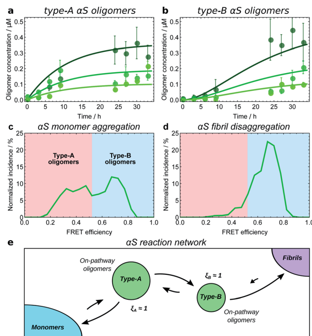
Fig. 7 Kinetic model fitting used to establish the reaction network for \alpha -synuclein monomers, oligomers and fibrils. Initial \alpha S monomer concentrations are 35, 70 and 140 \mu\text{M} (increasing darkness); oligomer concentrations measured by single-molecule FRET. 8 Data from ref. 25 (a and b), and ref. 8 (c and d). (a) Type-A \alpha S oligomers show initially-convex kinetic profiles, requiring a model in which they form directly from monomeric \alpha S. (b) Type-B \alpha S oligomers show initially-concave kinetic profiles, requiring a model in which they form by conformational conversion from type-A oligomers. (c) Distribution of oligomer FRET efficiencies halfway through an \alpha S aggregation reaction. Two peaks in the distribution can be seen, with the lower FRET peak corresponding to type-A oligomers, and the higher peak corresponding to type-B oligomers. (d) Distribution of oligomer FRET efficiencies near the start of an \alpha S fibril disaggregation reaction performed under similar reaction conditions, showing that only high-FRET type-B oligomers are produced directly from fibrils. Thus to satisfy the requirement of microscopic reversibility, new fibrils must be produced from type-B oligomers and not from type-A oligomers during aggregation. (e) The resultant reaction network; all oligomers are clearly on-pathway. Note the extent to which type-B oligomers convert back to type-A oligomers is not known; this is due to relatively large errors in oligomer concentration data at late times in the aggregation reaction.
