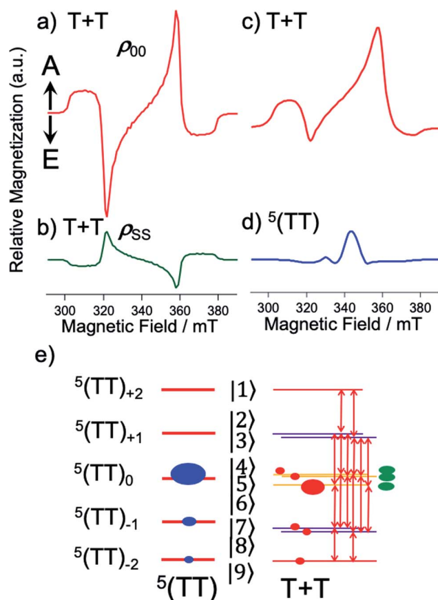
Fig. 5 Computed EPR spectra after the powder-pattern integrations of the T + T states (Fig. 4b) with D_{SS} = 0 and J = 0 in (a–c) and of the strongly-coupled {}^5(TT) in (d) using the ZFS interaction of {}^3TIPS -Pn. (a) {}^5(TT)_0 -precursor SCTP showing the A/E/A/E pattern and (b) {}^1(TT) -precursor case (Fig. 4b) resulting in the E/A/E/A pattern by the sequential ESPT model (green line in Fig. 7). (c and d) SCTP and strongly coupled {}^5(TT) polarization computed with eqn (13) from the spin-state populations \rho_{00}^{TT} = 0.75 , \rho_{-1-1}^{TT} = 0.19 , and \rho_{-2-2}^{TT} = 0.07 in {}^5(TT) in (e). (e) Computed T + T populations by eqn (15) are shown by red circles to explain the absorptive ESP in (c) and (d) corresponding to the 0.2 \mu s-spectrum in Fig. 3a. Sixteen allowed EPR transitions are shown to obtain the T + T spectra in (b) and (c) with the sublevel populations by the {}^1(TT) precursor (green) and by the {}^5(TT) precursor (red) from the blue circles, respectively.
