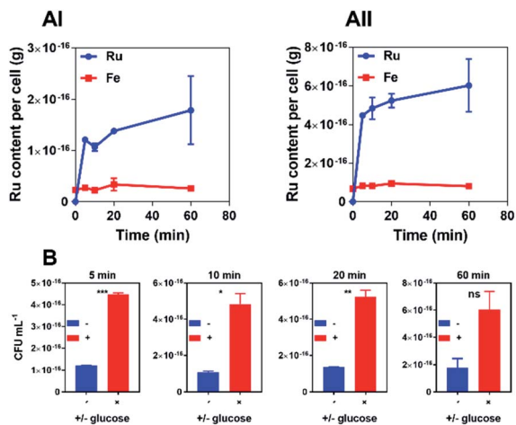
Fig. 3 Accumulation experiments. ICP-AES data for the uptake of ruthenium by S. aureus , SH1000, after exposure to 4^{4+} in the absence (A1) and presence (A2) of glucose. Ru (blue) and Fe (red) levels per cell are exposed as metal (g) per cell. T -test stats are given as a comparison at each time-point (B). Fe levels were calculated as a control. Conditions: concentration of 4^{4+} = 4 \mu M. Cells were washed with 0.5% (v/v) nitric acid to remove unbound complex. Error bars represent three independent biological repeats \pm SD.
