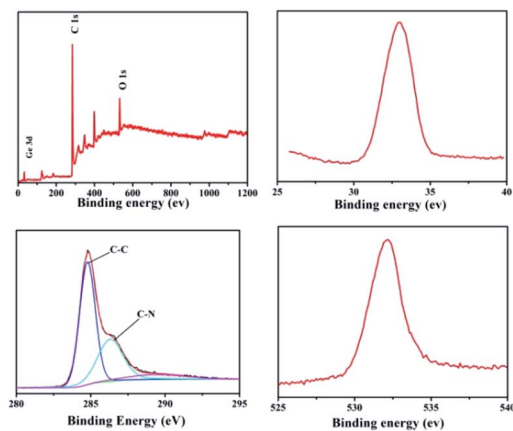
Fig. 2 XPS spectra of GeO 2 /nanocable: (a) the full XPS spectrum of the GeO 2 /nanocable; (b–d) high-resolution spectra Ge 3d, C 1s and O 1s, respectively.
