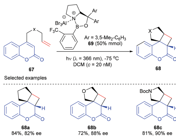
Scheme 19 Chiral AlBr 3 complex catalyzed enantioselective [2 + 2]-cycloaddition reactions.
