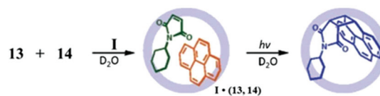
Fig. 32 [2 + 2] photo-addition of 13 and 14 within cage I . Reproduced with permission from ref. 118. Copyright 2007, American Chemical Society.
