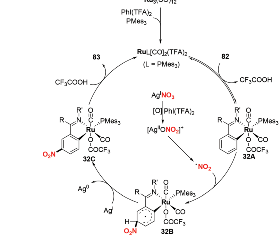
Scheme 32 Ruthenium-catalyzed PMe 3 -promoted meta -C-H nitration of arenes.
