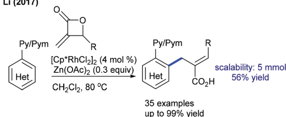
Scheme 137 Redox-neutral coupling of methylenexetanones with arenes.
