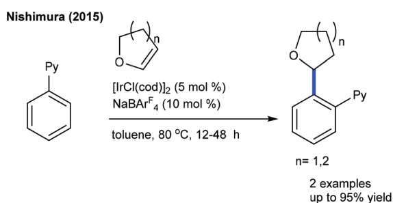
Scheme 52 Hydroarylation of cyclic ethers.
