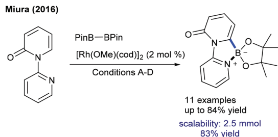
Scheme 103 C6-Borylation of pyridones.
