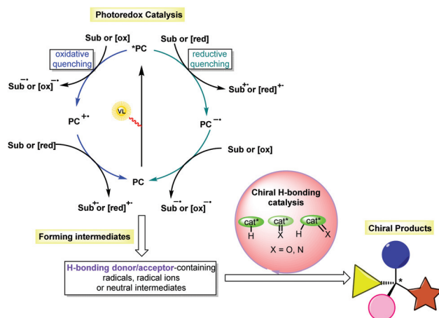
Scheme 1 Cooperative asymmetric and H-bonding catalysis.
