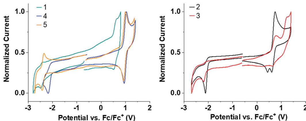
Fig. 3 Normalized CV redox curves for 1–5 in deoxygenated MeCN solvent. All curves are referenced to the \text{Fc}/\text{Fc}^+ redox couple.
