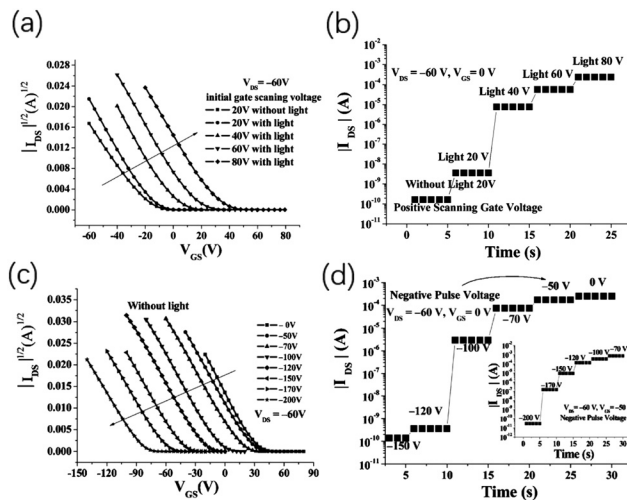
Fig. 14 I – V curves of devices with light-assisted programming (the initial scanning gate voltage is V_{G,Start} = 20 V, 40 V, 60 V, and 80 V, V_D = -60 V, and with the visible-light intensity increased with the arrowhead). (a) |I_D|^{1/2} versus V_G and (b) the corresponding different current levels at V_G = 0 V and V_D = -60 V in the process for OFETs with a PS modifying layer. (c) Different transfer characteristics of the devices using voltage programming ( V_{G,Pro} = -50 V, -70 V, -100 V, -120 V, -150 V, -170 V, and -200 V, V_D = 0 V, t = 1 ms) without light, and (d) the corresponding different current levels at V_G = 0 V, V_D = -60 V and V_G = -50 V, V_D = -60 V (inset graph) in the process. Reproduced with permission. 83 Copyright 2009, John Wiley and Sons.
