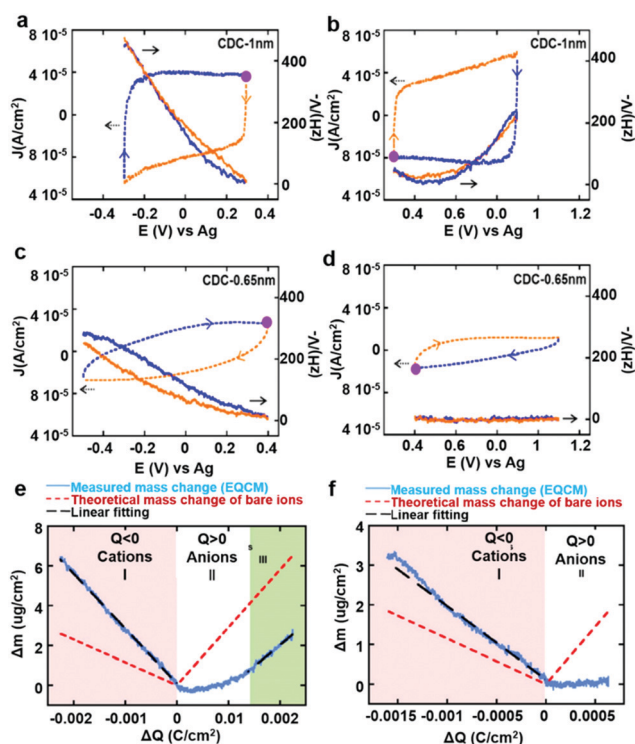
Fig. 8 CV and EQCM frequency response of (a and b) CDC-1 nm and (c and d) CDC-0.65 nm in 2 M EMI-TFSI/AN below (a and c) and above (b and d) the immersion potential (the purple dot is where the cycle starts; orange and blue curves indicate charge and discharge of ions, respectively). Electrode mass change vs. charge during the polarization of (e) CDC-1 nm and (f) CDC-0.65 nm in 2 M EMI-TFSI + AN (blue solid lines are measured mass change (EQCM); red dashed lines are the theoretical mass change of neat ions calculated from Faraday's law and the black dashed line shows the linear fitting of measured mass change). Reproduced with permission from ref. 46. Copyright 2014 American Chemical Society.
